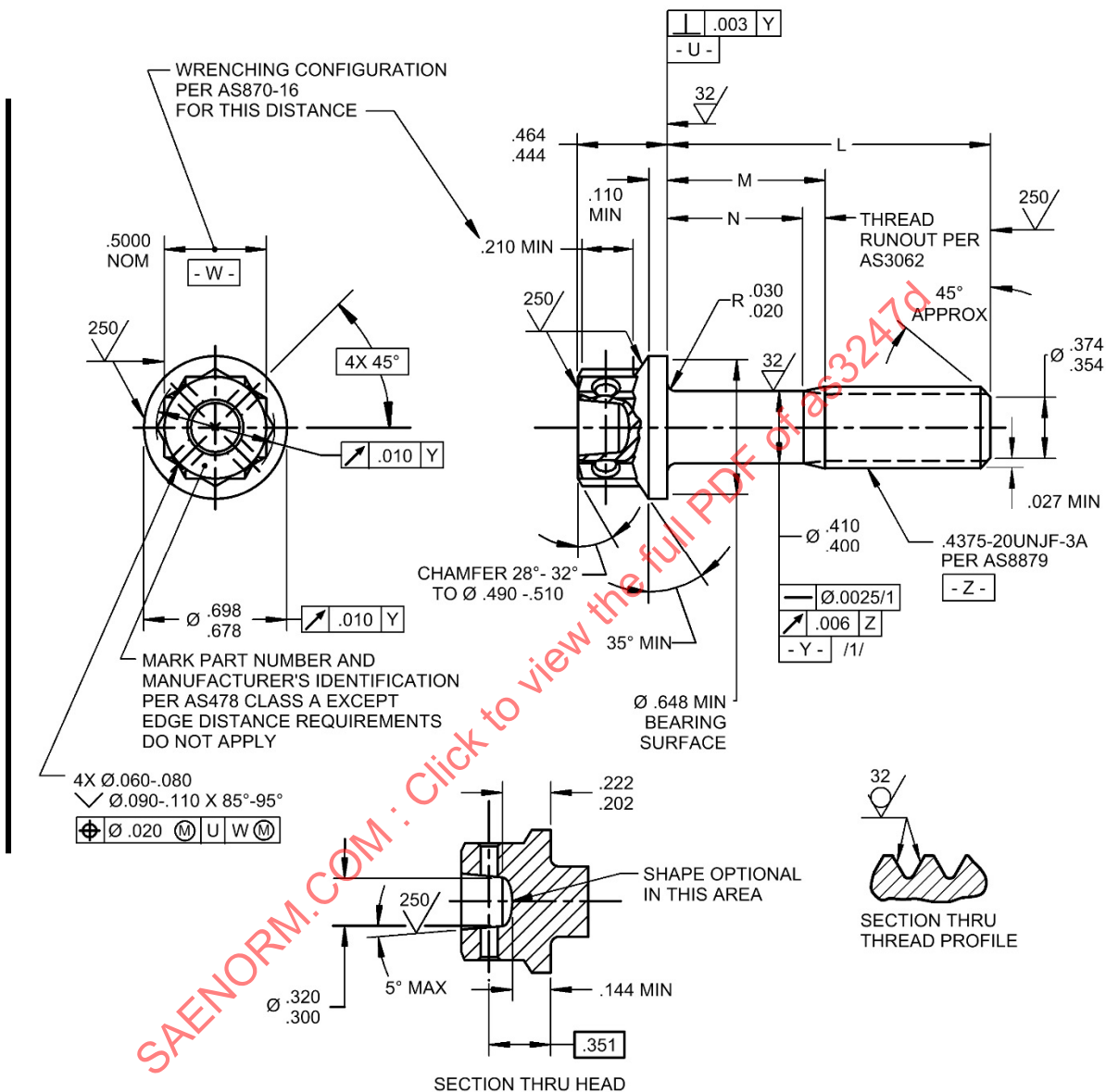
FIGURE 1 - BOLT
