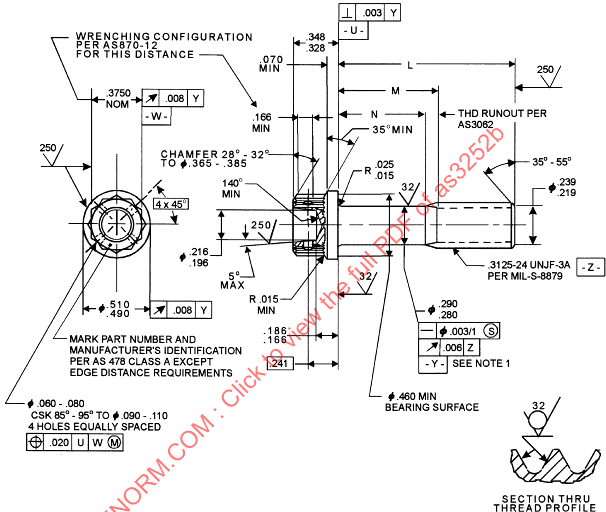
FIGURE 1 - BOLT
