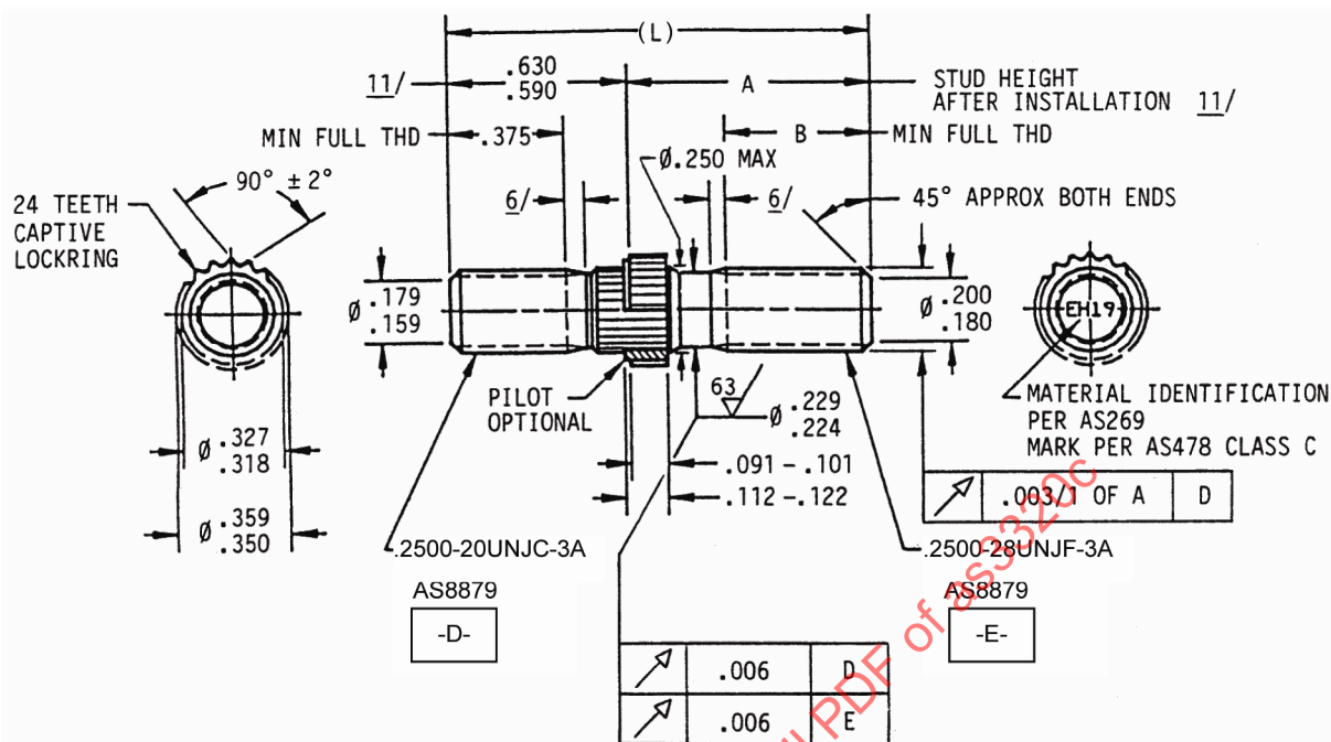
FIGURE 1 - STUD
