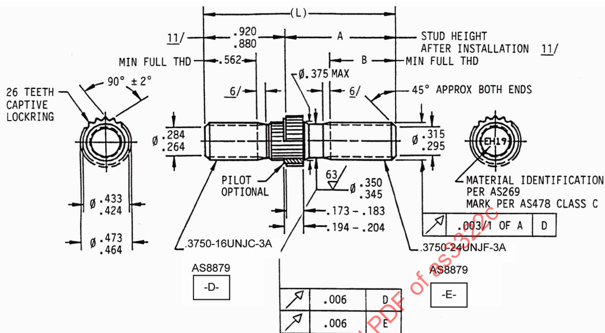
FIGURE 1 - STUD
