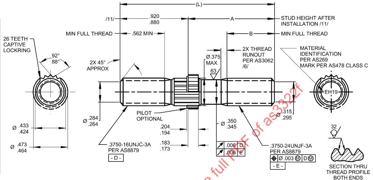
FIGURE 1 - STUD
