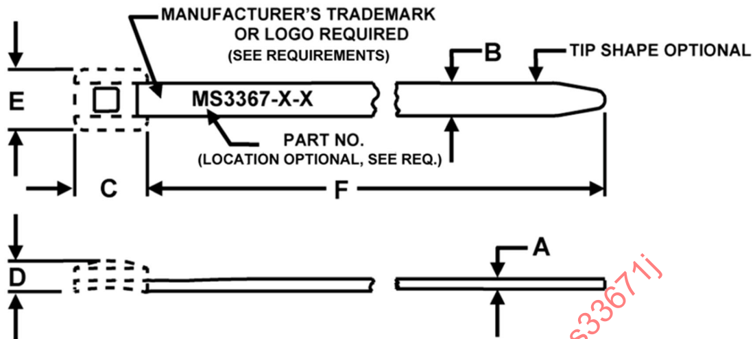
FIGURE 2 - STRAP CONFIGURATIONS/DIMENSIONS
