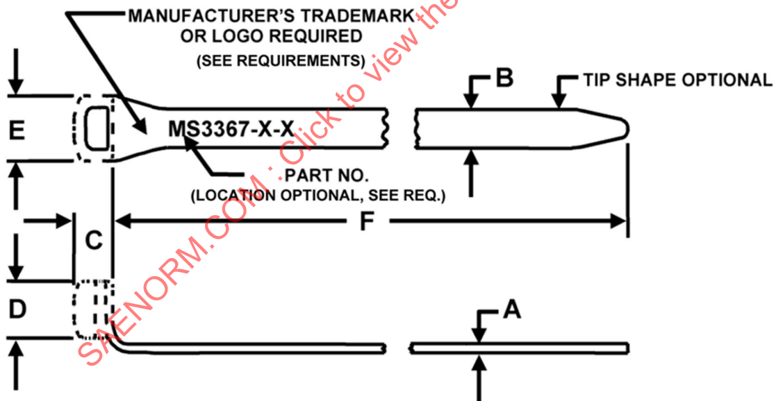
FIGURE 3 - STRAP CONFIGURATIONS/DIMENSIONS
