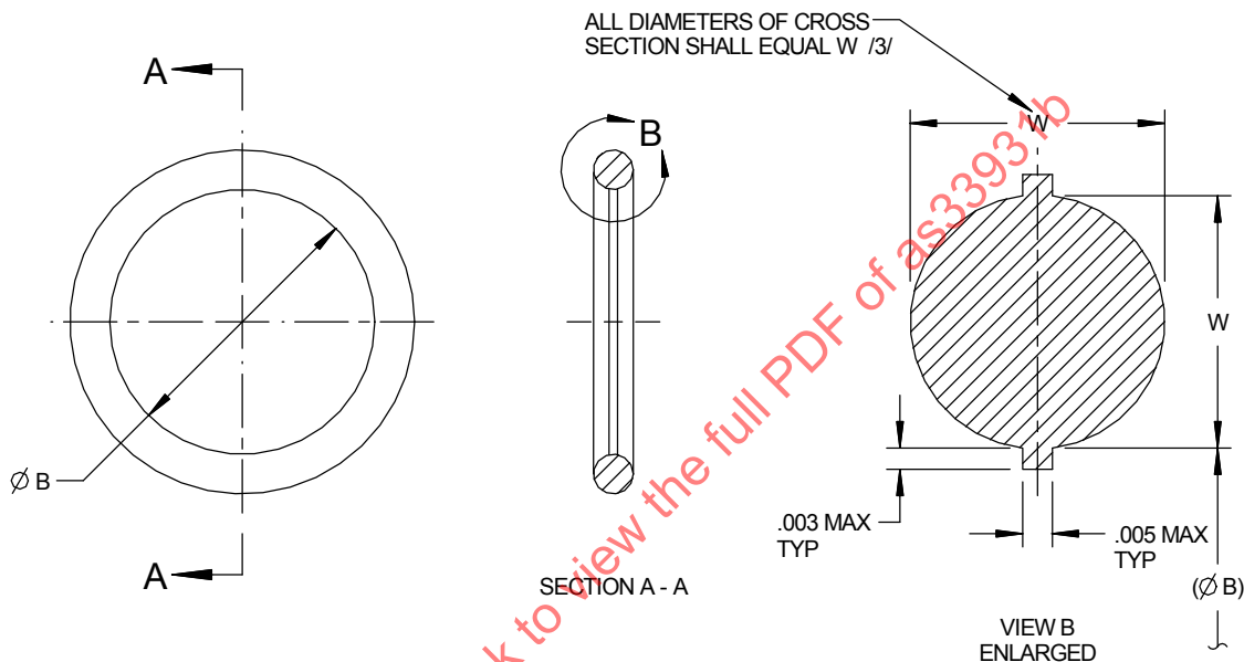
FIGURE 1 - PACKING, PREFORMED
