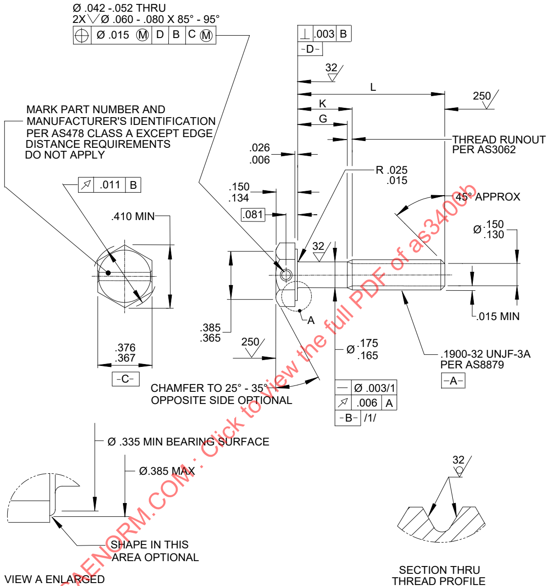
FIGURE 1 - BOLT
