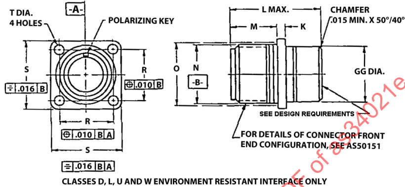
FIGURE 1 - CONNECTOR CONFIGURATION AND DIMENSIONS
