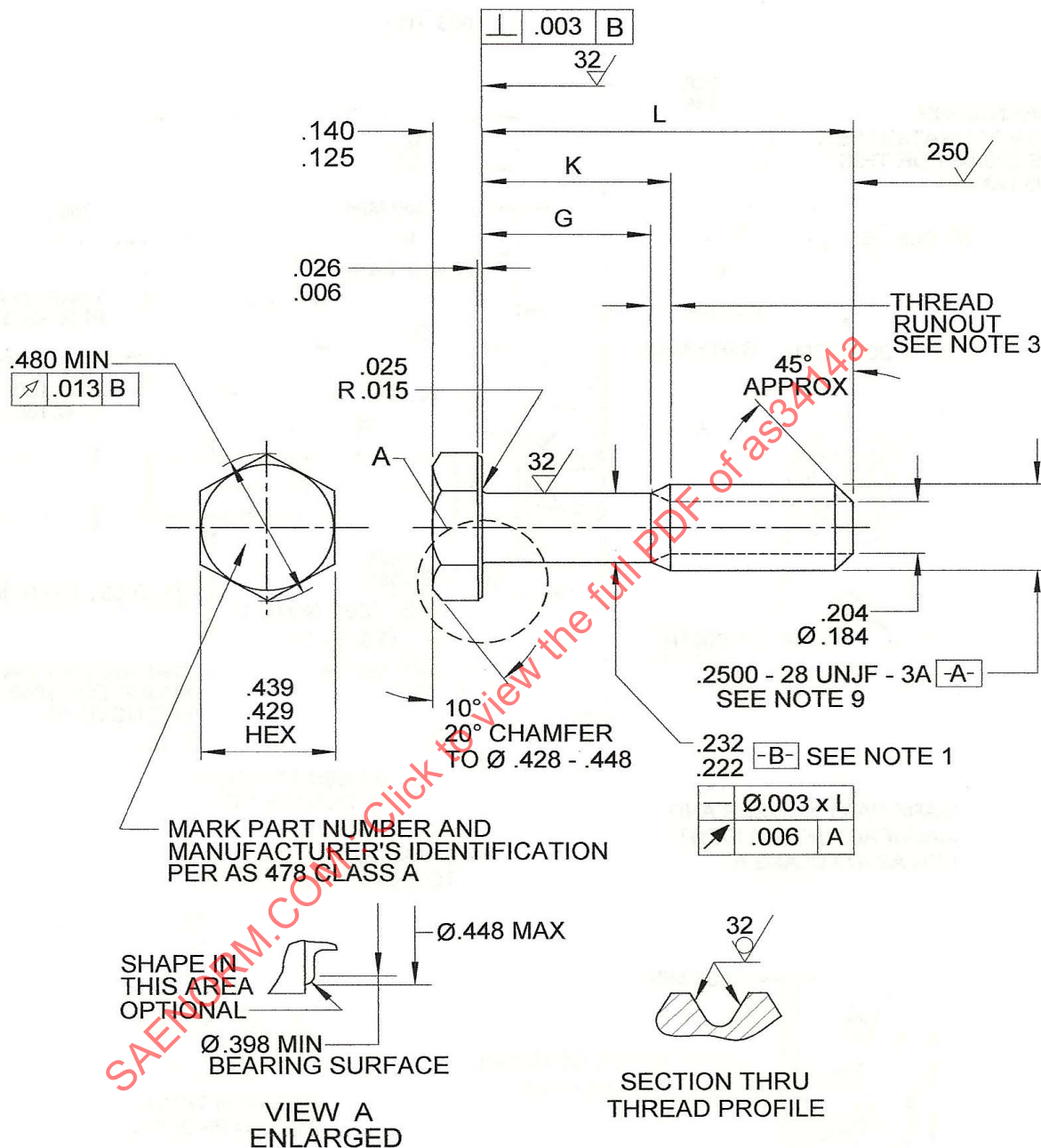
FIGURE1 - BOLT
