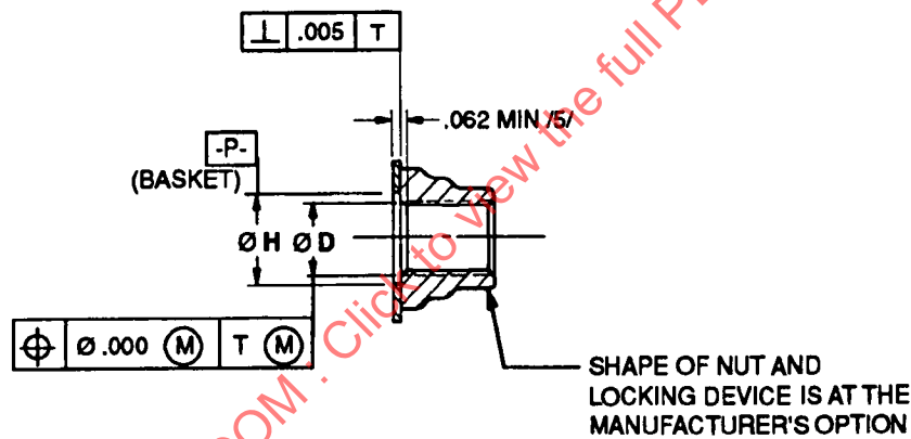
SECTION L-L
