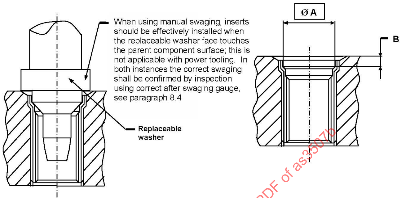
FIGURE 6 - Swaging of Insert
