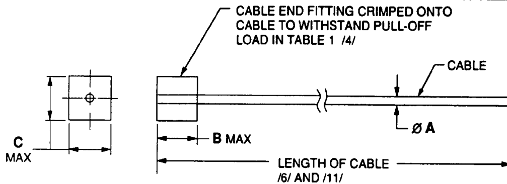
FIGURE 1 - SAFETY CABLE-END FITTING AND CABLE ASSEMBLY
