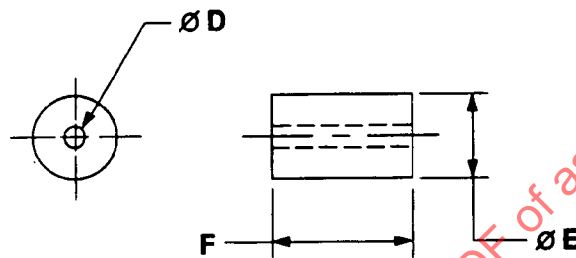
FIGURE 2 - FERRULE
