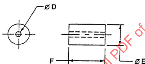
FIGURE 2 - FERRULE
