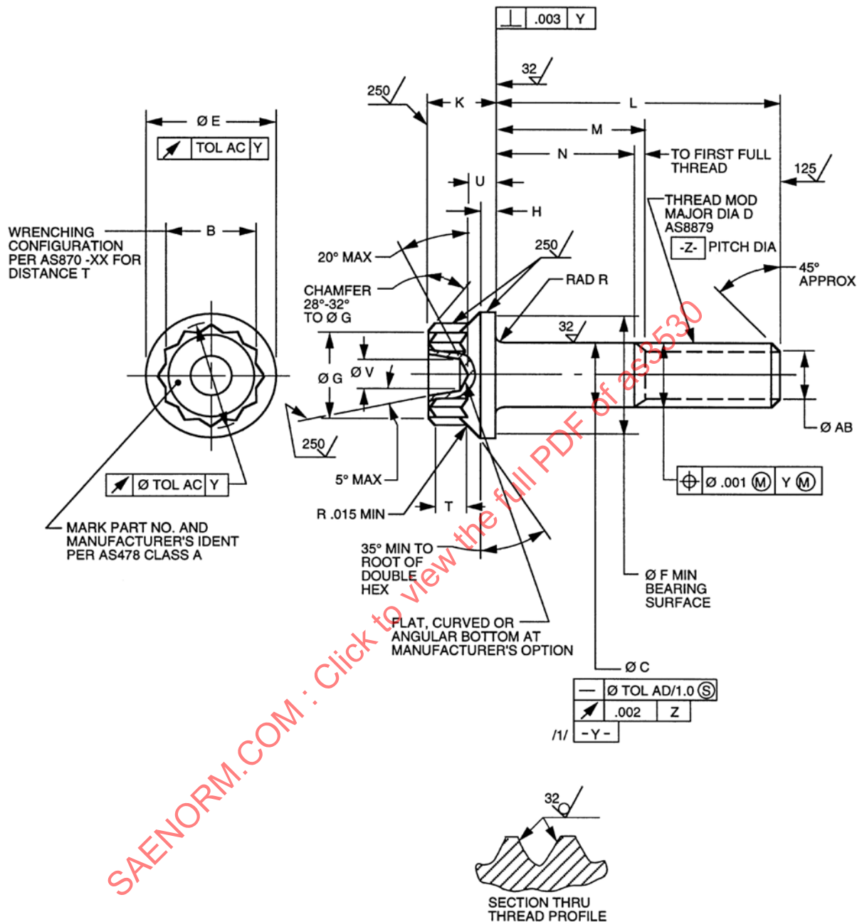
FIGURE 1 - MACHINE BOLT
