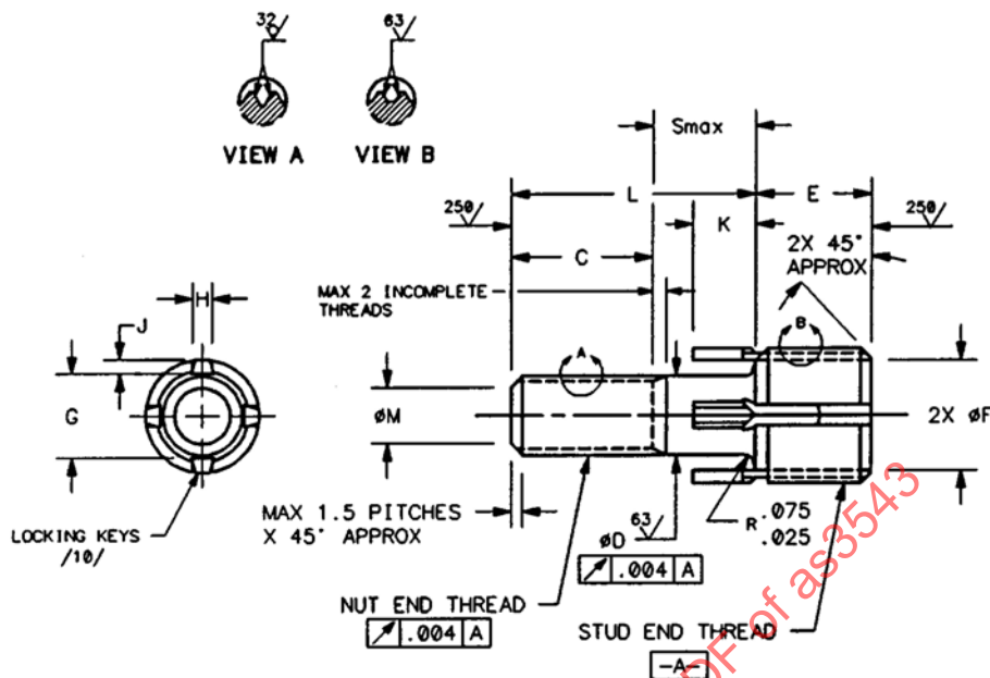
FIGURE 1 - STUD, FINE THREAD, NUT END
