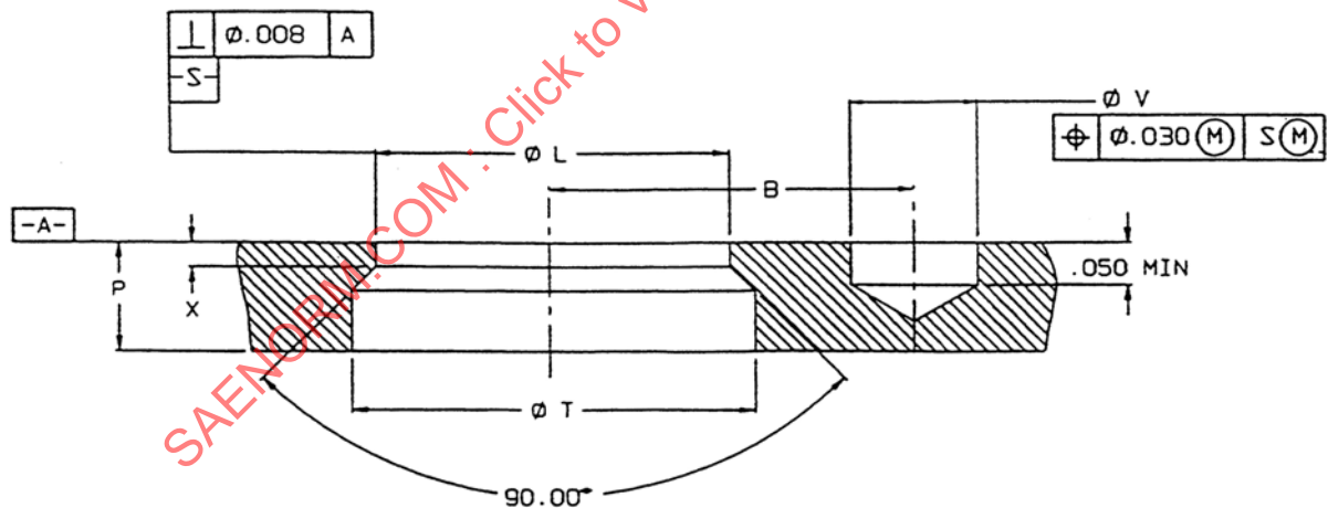
FIGURE 2 - INSTALLATION HOLE
