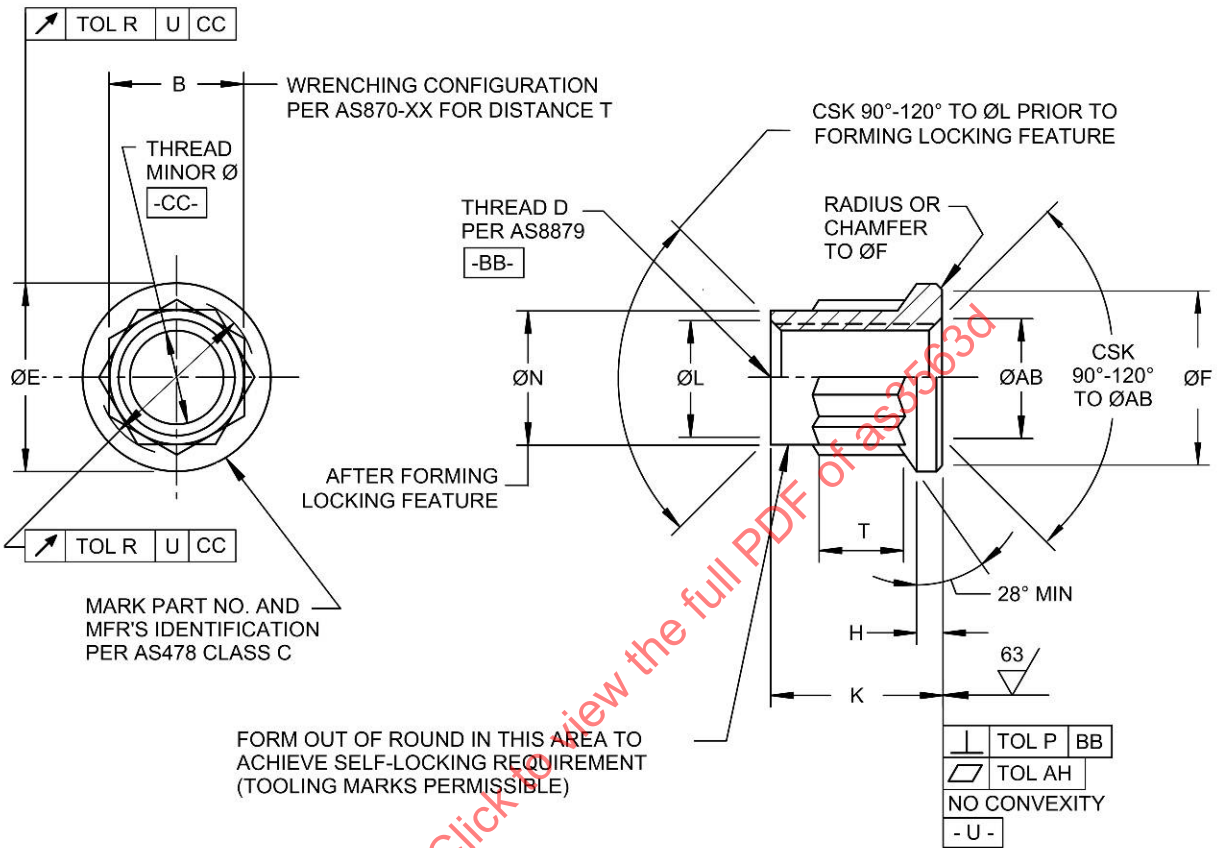
FIGURE 1 - NUT
