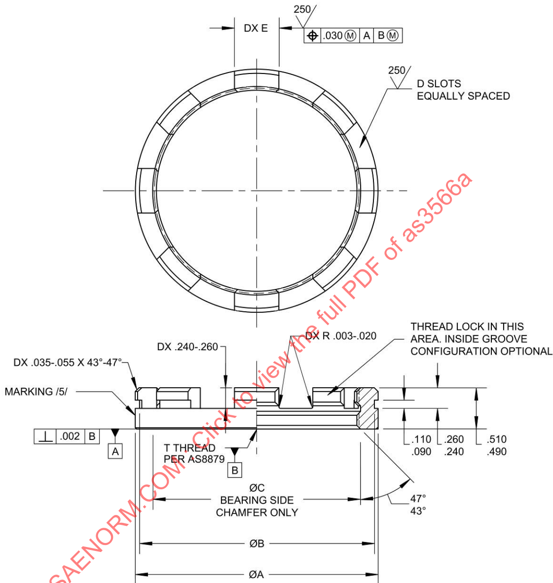
FIGURE 1 - NUT
