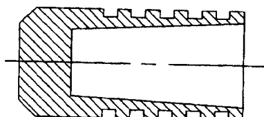
FIGURE 2 - AS3125 PLUG
