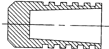
FIGURE 2 - AS3125 PLUG
