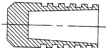
FIGURE 2 - AS3131 PLUG
