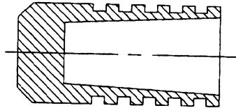
FIGURE 2 - AS3123 PLUG
