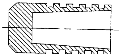
FIGURE 2 - AS3121 PLUG
