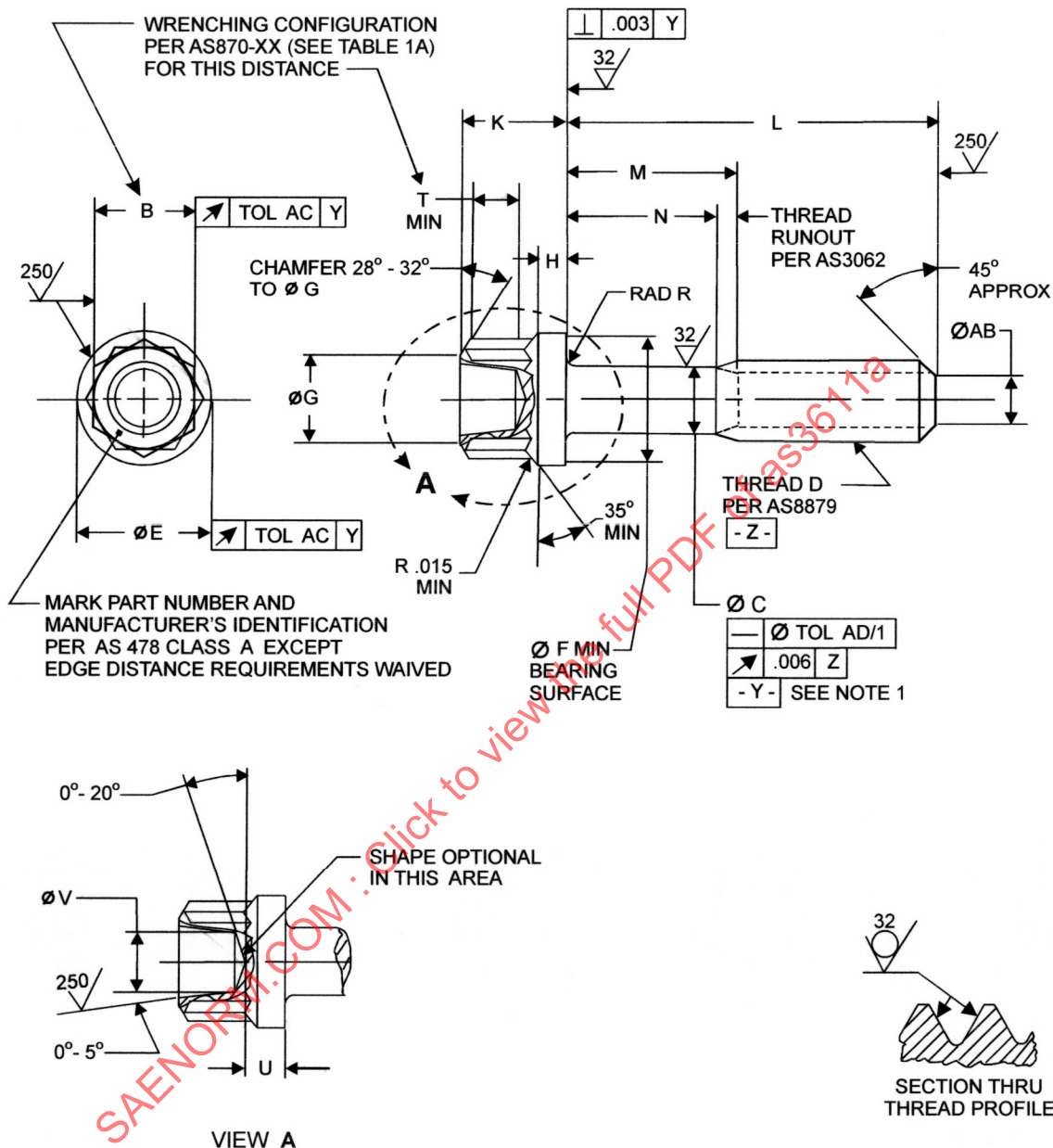
FIGURE 1 – BOLT
