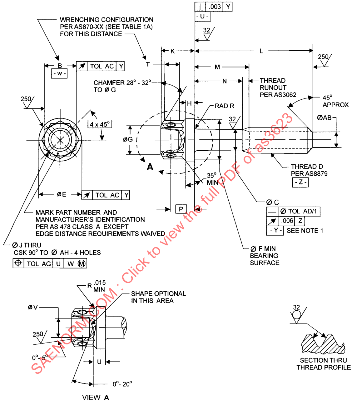
FIGURE 1 - BOLT
