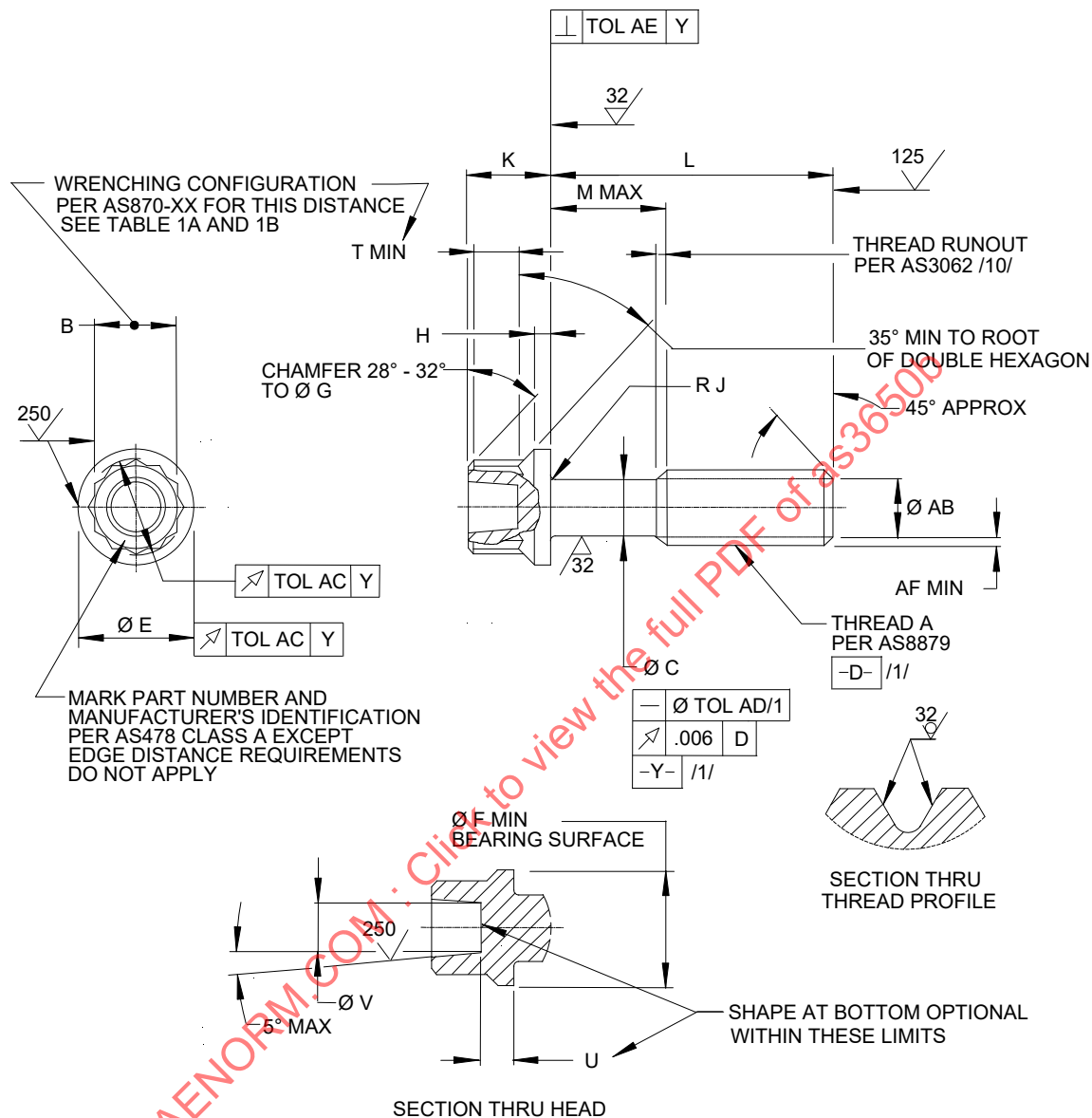
FIGURE 1 - BOLT
