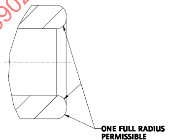
FIGURE 1- AS39029/106 SOCKET (CONTINUED- SEE DESIGN REQUIREMENTS)
