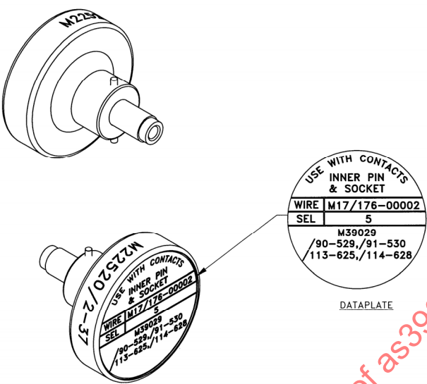
FIGURE 1 - GRAPHIC OF M22520/2-37 POSITIONER
