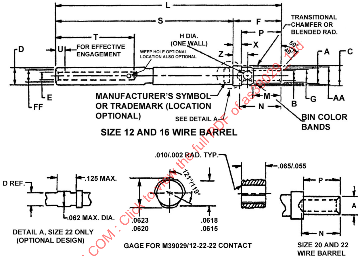
FIGURE 1 - SOCKET CONTACT
