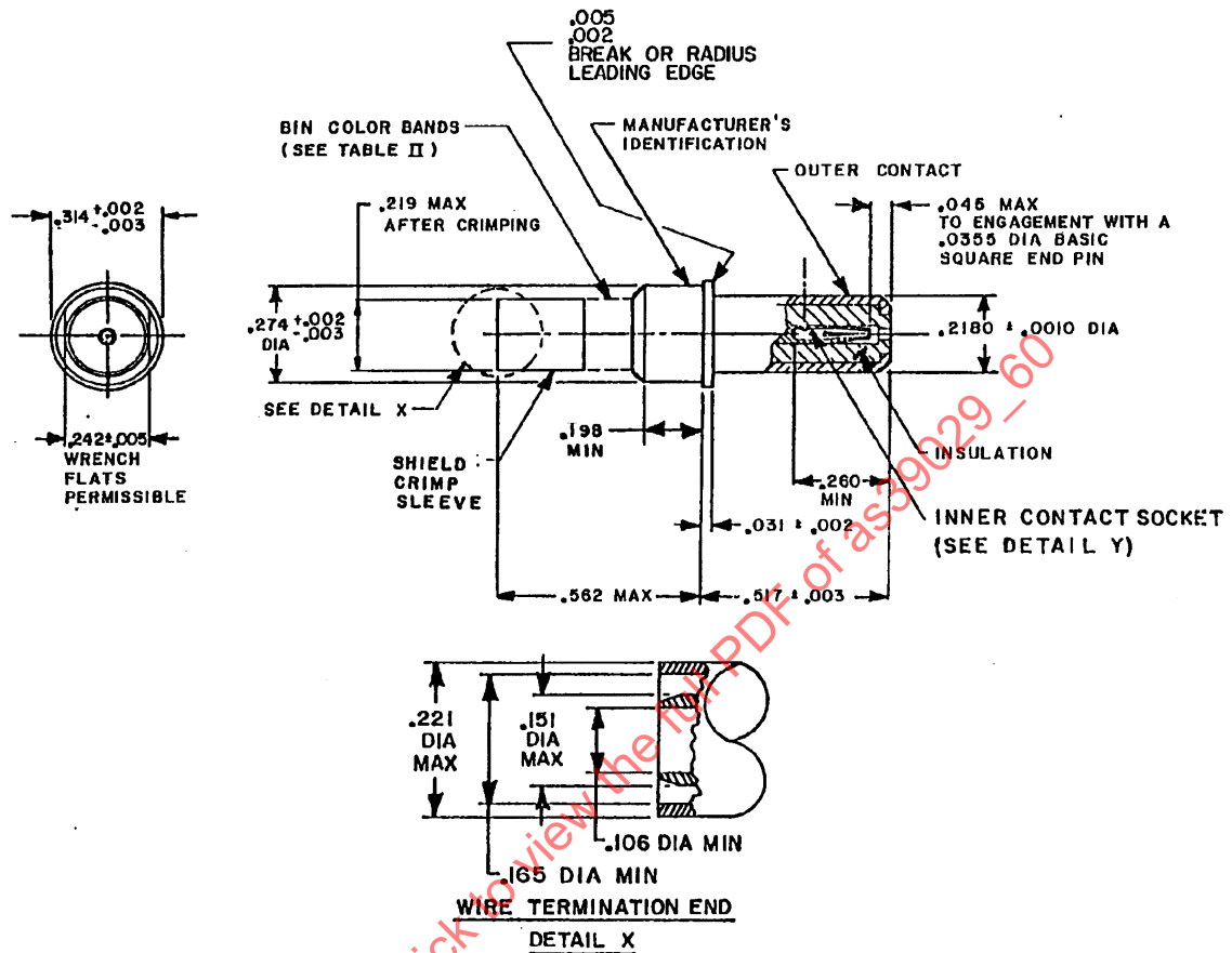
FIGURE 1. CONNECTOR CONTACT.
