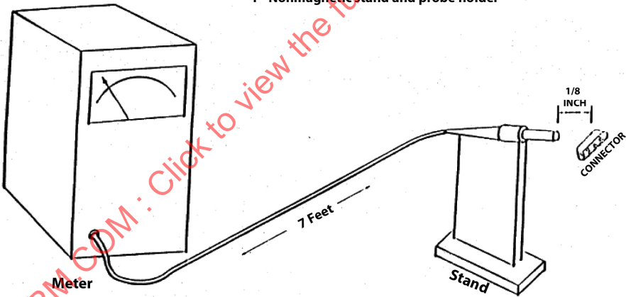
FIGURE 2 - RESIDUAL MAGNETISM TEST ARRANGEMENT
