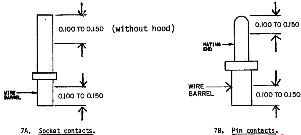
FIGURE 7 - PLATING THICKNESS MEASUREMENT - OVERALL FINISH (TYPES A, B AND D)
