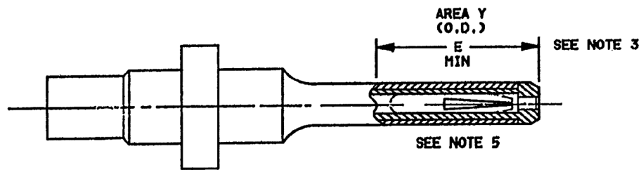
2A. Outer pin contact.
