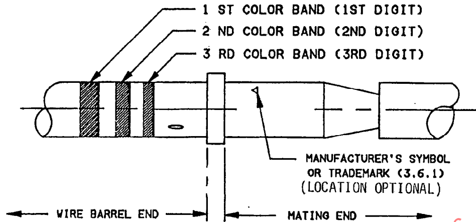
FIGURE 3 - CONTACT MARKING
