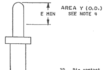
1D. Pin contact.
