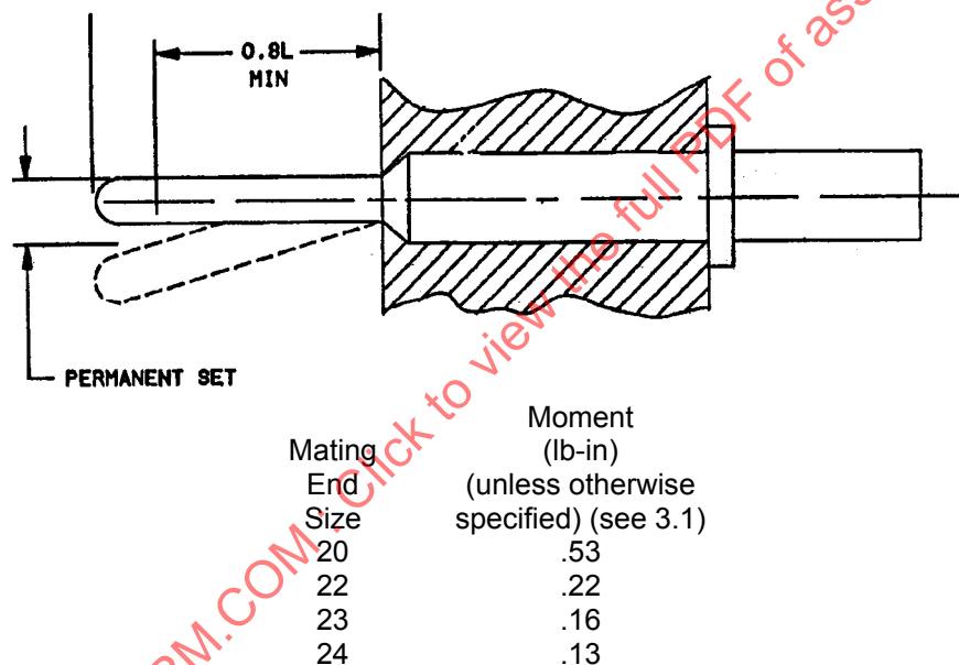
FIGURE 6 - CONTACT STRENGTH (TYPICAL)
