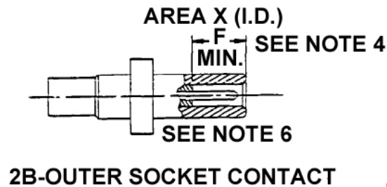
Figure 3 - Areas of application of localized finish (Type D outer contacts)
