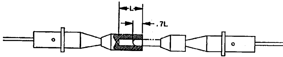
Figure 6 - Depth of engagement for contact resistance and engagement and separation force tests
