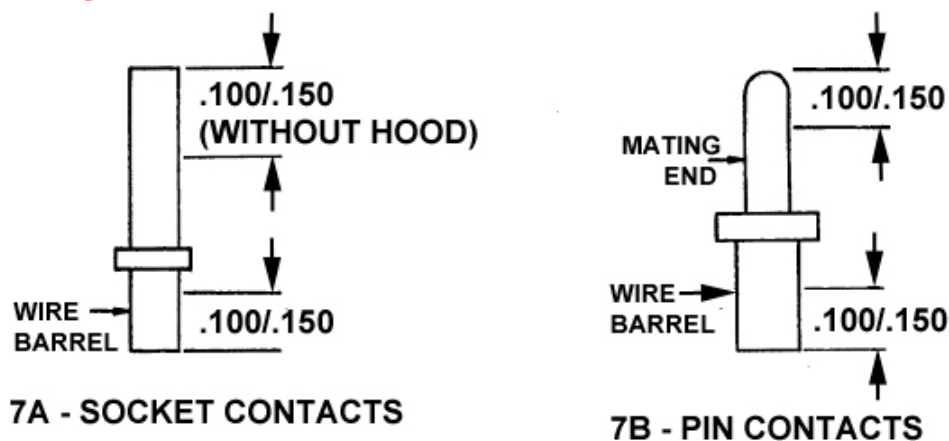
Figure 8 - Plating thickness measurement - overall finish (Types A, B, and D)
