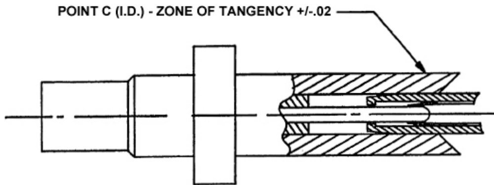
9A. SOCKET CONTACT - OUTER WITH INTEGRAL PRESSURE MEMBERS PIN CONTACT - INNER (SEE FIGURE 8)
