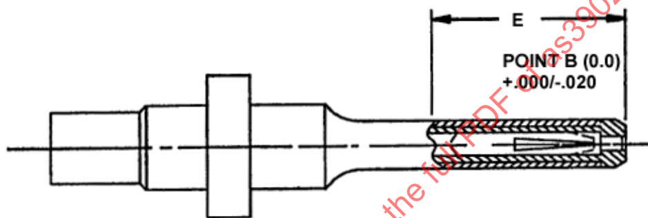
9B. PIN CONTACT - OUTER SOCKET CONTACT - INNER (SEE FIGURE 8)
