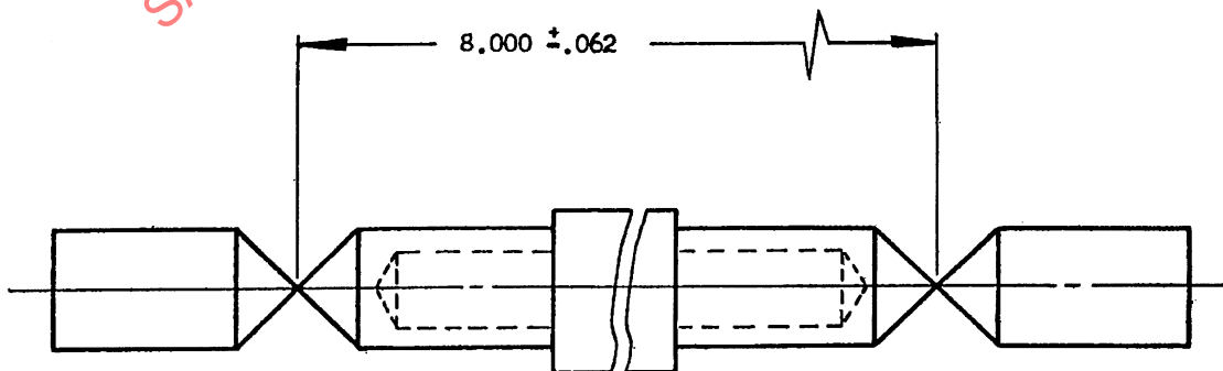
FIGURE 2. Specimen for fatigue, friction torque, and operability test.
