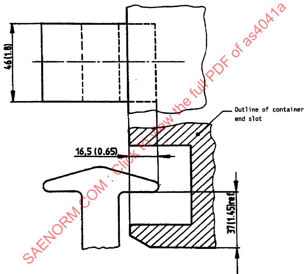
FIGURE 7 - End Latch Dimension
