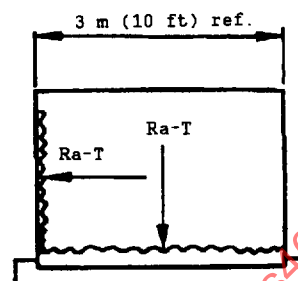
Test No. 1.2 - Strength of End Wall/Door - Forward Operational Load - 1D Container Only
