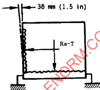
Test No. 2.1 - Strength of End Sidewalls - Side Operational Load
