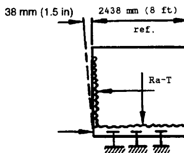
Test No. 2.2 - Strength of End Sidewalls - Side Operational Load - 1D Container Only
