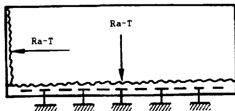
Test No. 1.1 - Strength of End Wall/Door - Forward Operational Load
