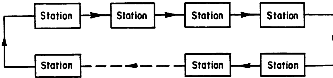
FIGURE 3.1-1 - Single Ring
