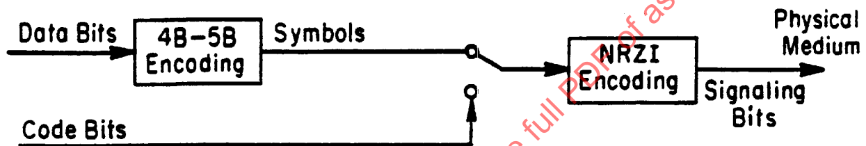
FIGURE 3.4.1-1 - Signaling And Code Bits
