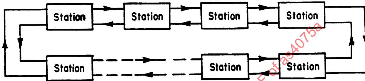
FIGURE 3.1-2 - Dual Ring
