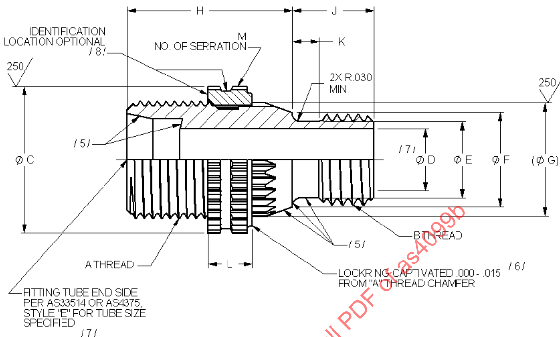
FIGURE 1 - ADAPTER, ASSEMBLY
