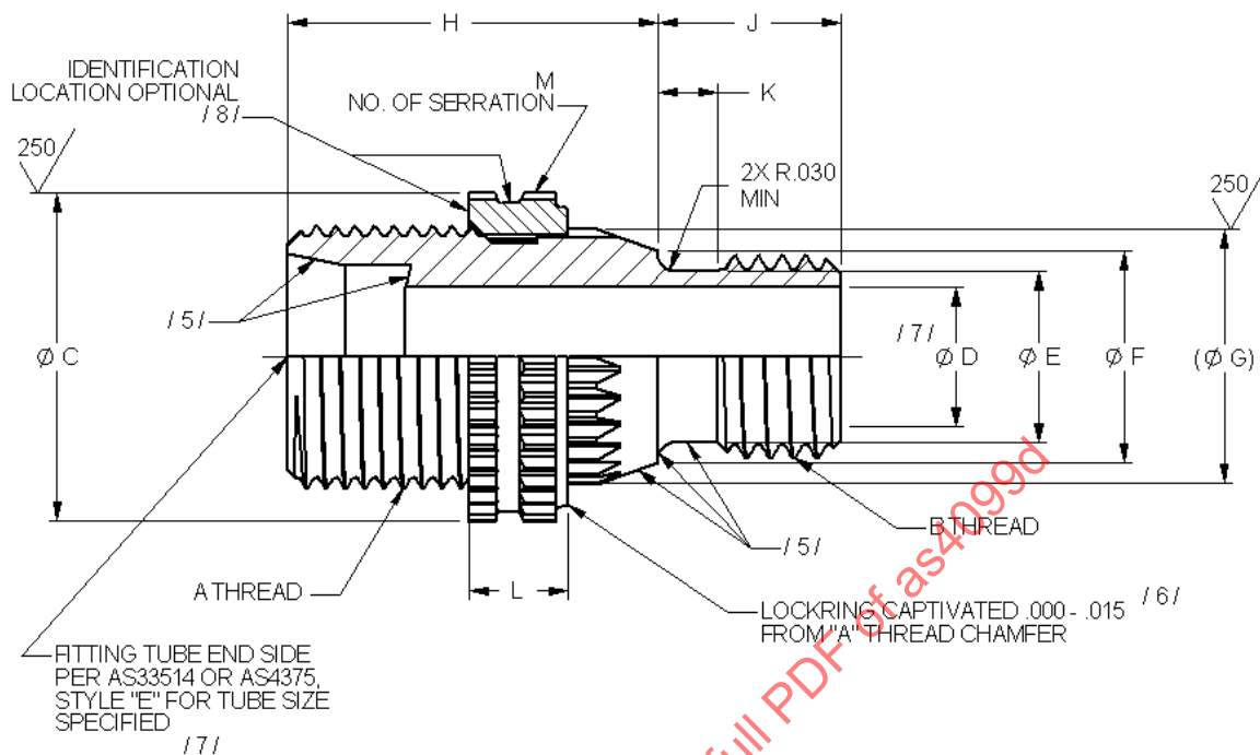
FIGURE 1 - ADAPTER ASSEMBLY
