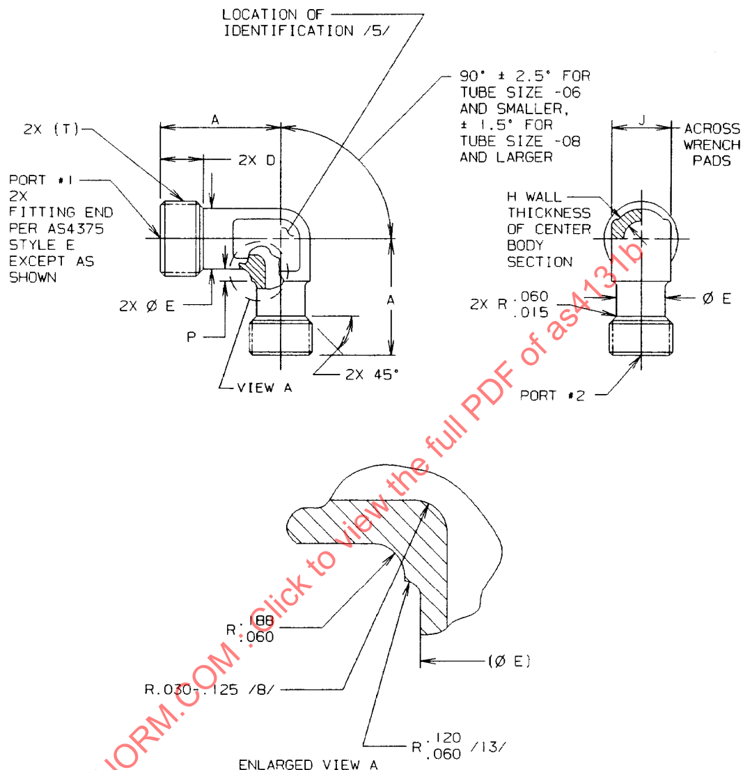
FIGURE 1 – ELBOW, 90 DEGREE, REDUCED BODY, FLARELESS
