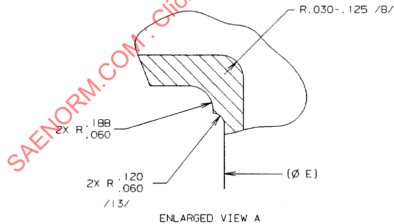
FIGURE 1 - TEE, REDUCED BODY, FLARELESS
