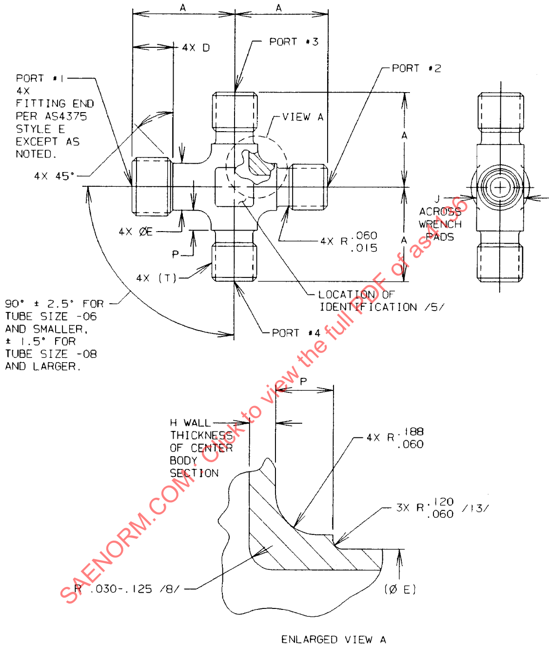
FIGURE 1 - CROSS, REDUCED BODY, FLARELESS
