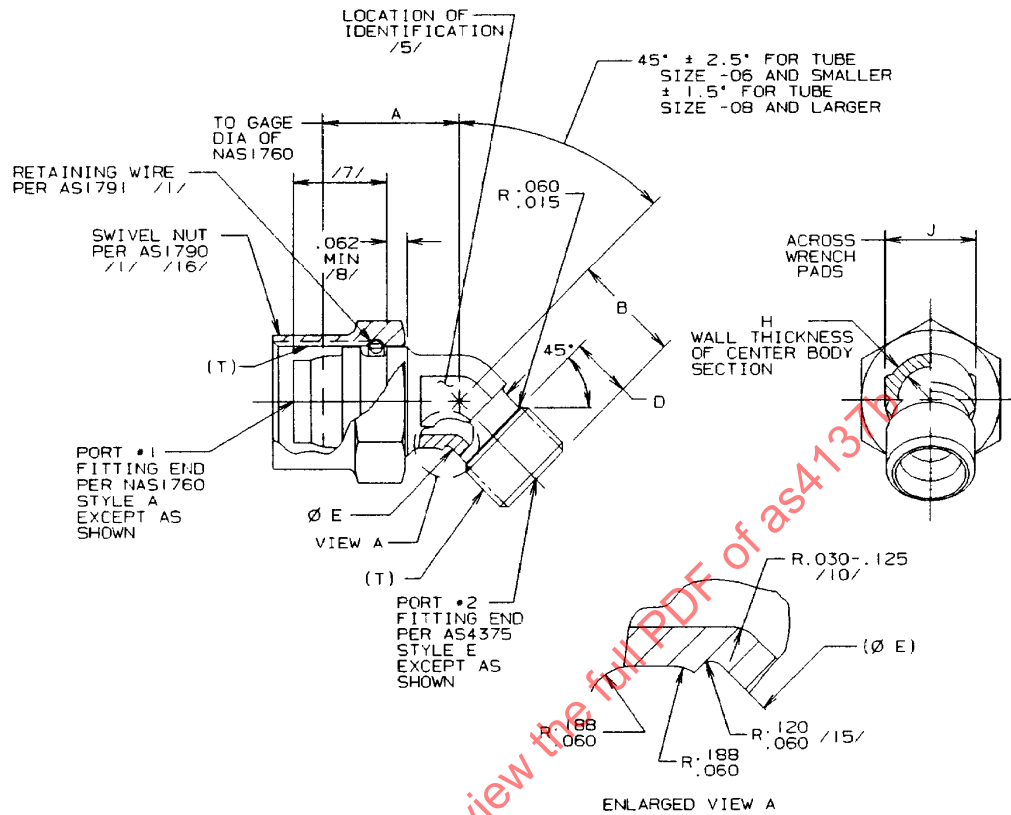
FIGURE 1 - FITTING ASSY, ELBOW, REDUCER, 45°, SWIVEL, REDUCED BODY, FLARELESS
