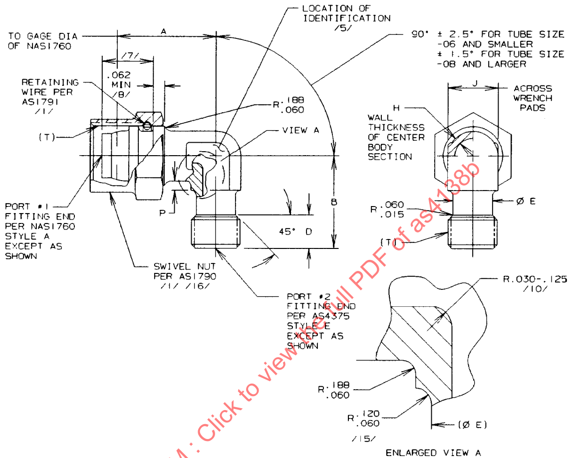
FIGURE 1 - FITTING ASSY, ELBOW, REDUCER, 90°, SWIVEL, REDUCED BODY, FLARELESS
