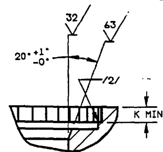
VIEW Z
