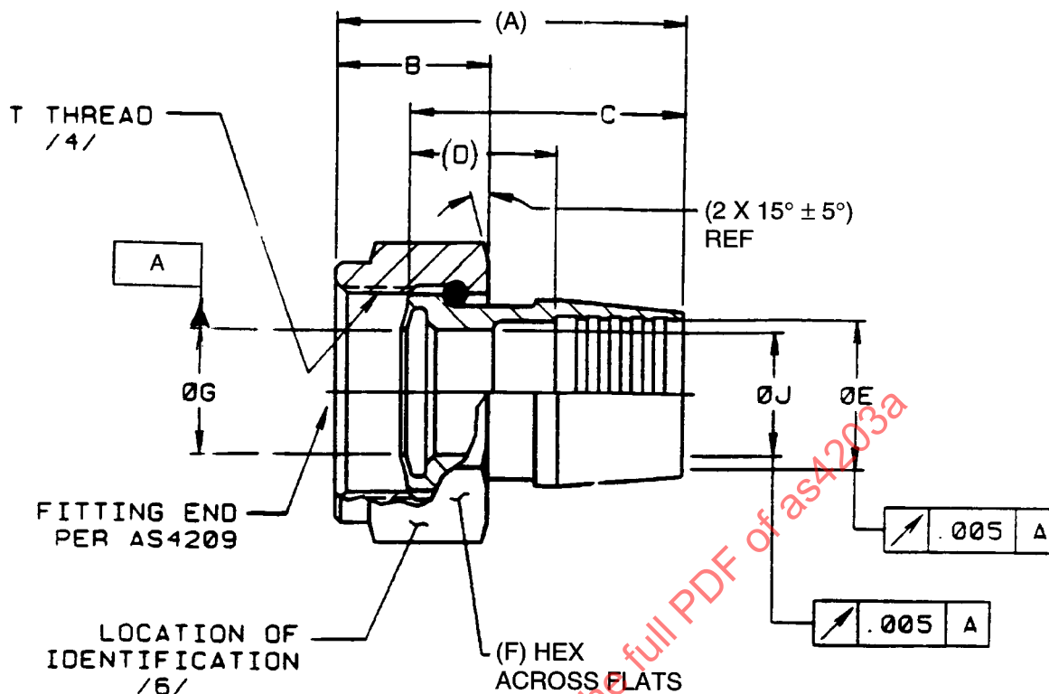
FIGURE 1 - FITTING ASSEMBLY (R) TABLE 1A - DIMENSIONS A-F
