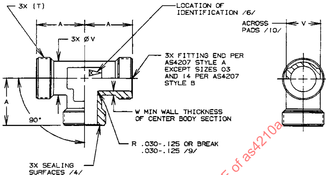
FIGURE 1 - FITTING, TEE
