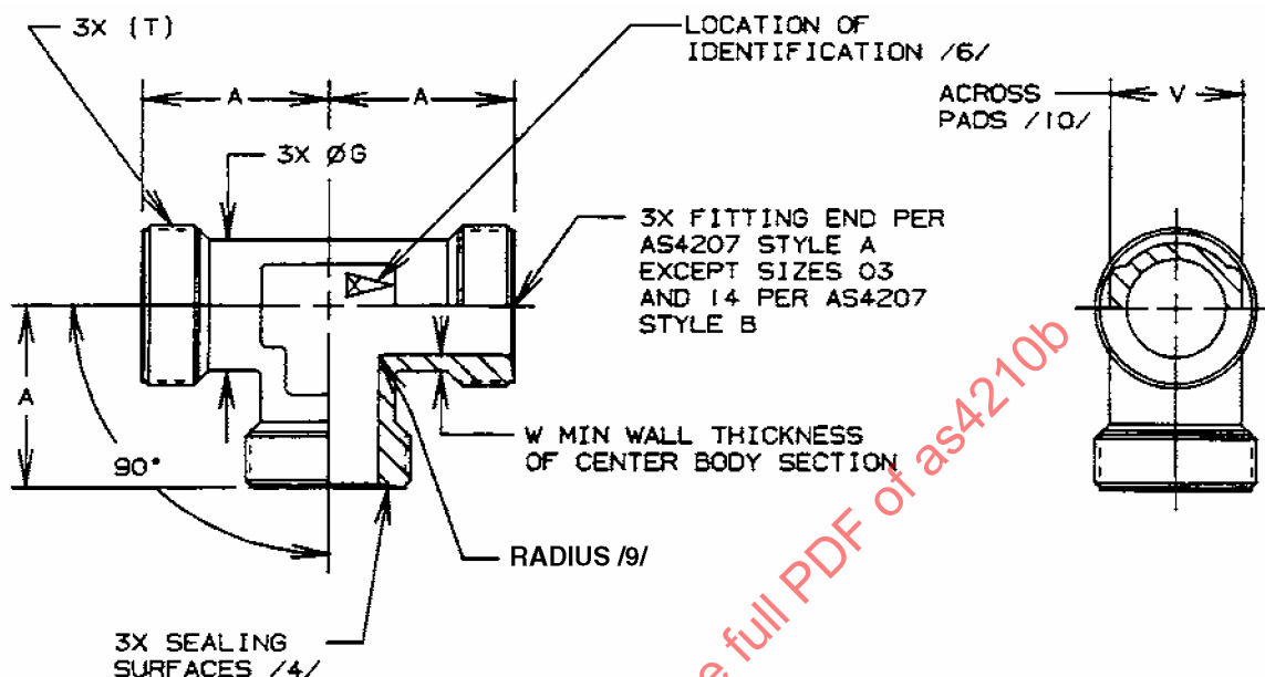
FIGURE 1 - FITTING, TEE
