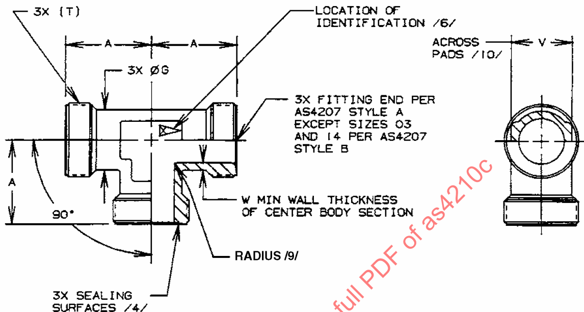
FIGURE 1 - FITTING, TEE
