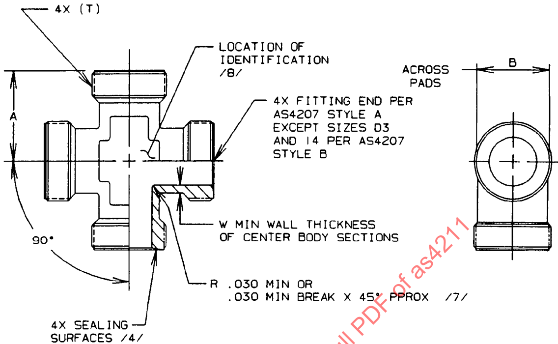
FIGURE 1 - CROSS, BEAM SEAL MALE
